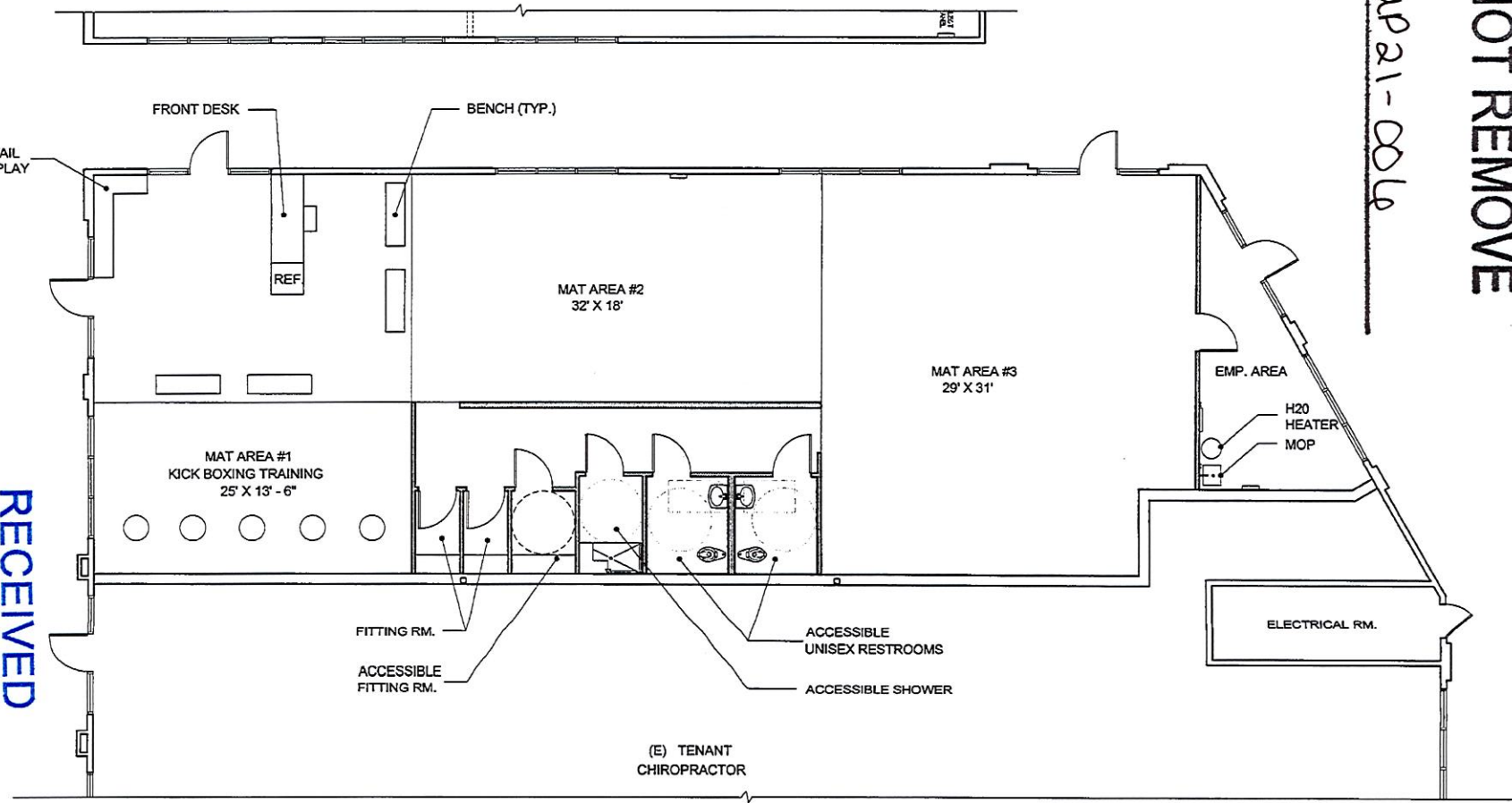
BUILDING B - FLOOR PLAN
