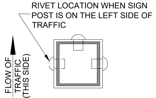
RIVET LOCATION SECTION A-A
