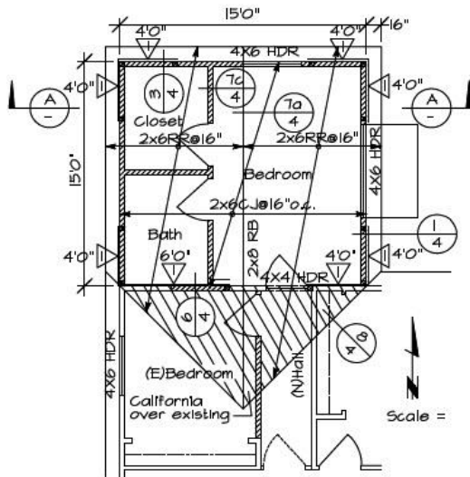
EXAMPLE FRAMING PLAN
