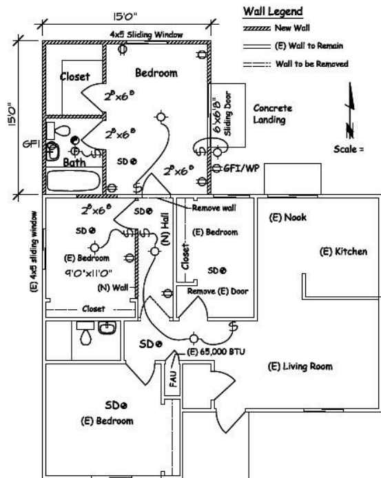
EXAMPLE FLOOR PLAN
