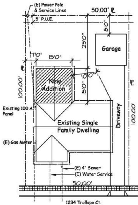
EXAMPLE PLOT PLAN
